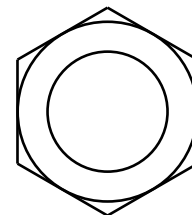
HEX NUT 5/8-11 BRASS
